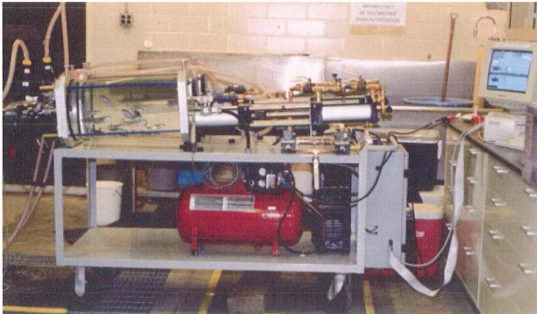
Figure 6. Turbine Passage System with Rainbow Trout in Hyperbaric Chambers (Abernethy et al. 2000)
