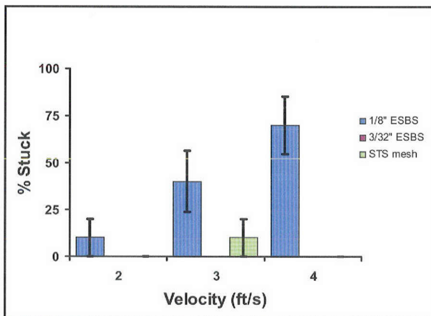
Figure 11. Lamprey Response to Three Types of Screens Material. Tests were conducted with screens perpendicular to the flow for 10-min durations ( n=20 for each 1/8-in. ESBS and n=10 for 3/32-in. ESBS and STS tests). Note that no lamprey became permanently stuck on the 3/32-in. bar screen (bars = \pm SE).
