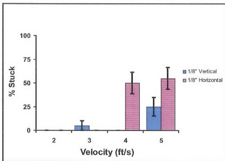
Figure 10. ESBS Screen Material Orientation Effects, Vertical and Horizontal, with a 10^\circ Degree Tilt to Simulate Sweeping Flows (bars = \pm SE, n=10)
