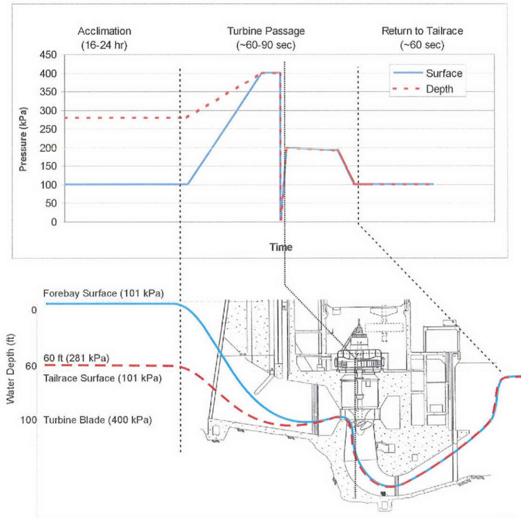
Figure 7. Diagram of Surface and 60-ft Depth Acclimation and Hyperbaric Chamber Pressure Exposure Simulation of Turbine Passage are Shown. Lamprey were acclimated at the 60-ft depth level.
