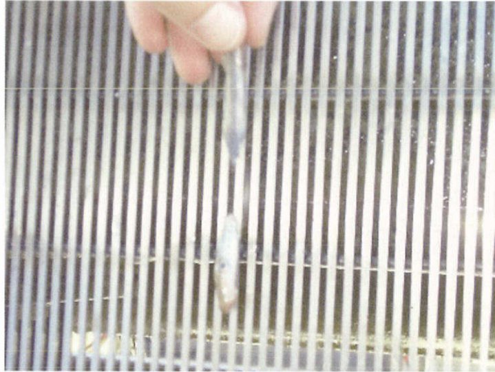
Figure 17. Lamprey Impinged on Screen 6B McNary Dam
