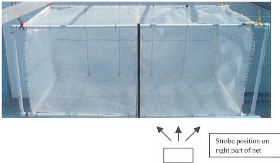
Figure 3. Static Strobe Test Net Pen with Light Position at Right Half of Pen
