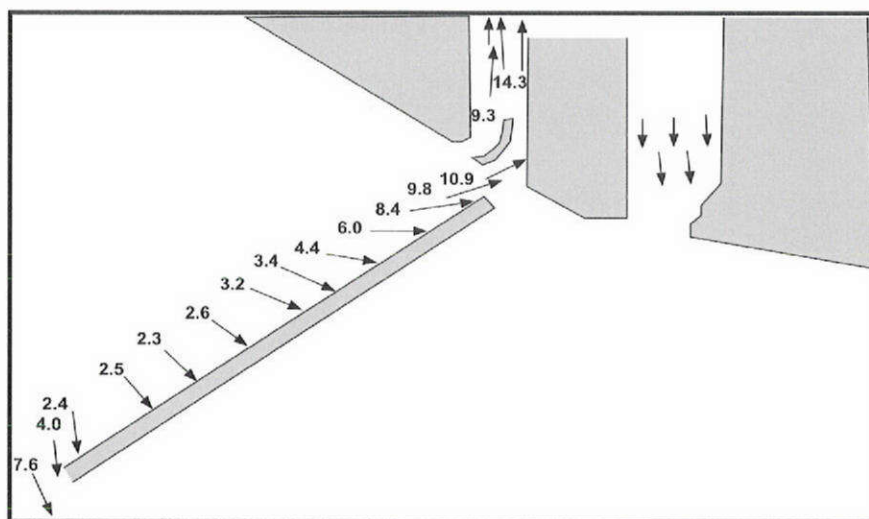
Figure 2. Cross-Section Diagram of the Velocity Vectors at a Deployed ESBS (John Day Dam) Based on Physical Model Data from the Corps
