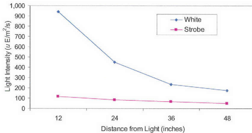
Figure 5. Strobe and White Light Intensities Measured at 12-in. Intervals Within the Swim Chamber
